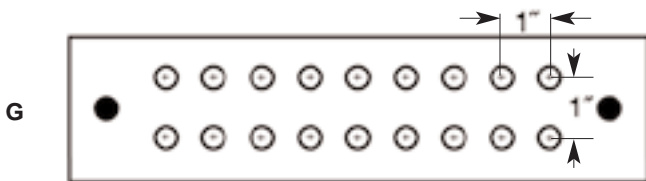
(18) lug-mounting holes (3/8 bolt size), for (9) 2-hole lugs (1 inch spacing), or (18) 1-hole lugs
